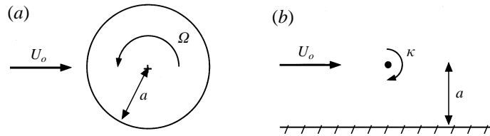
FIGURE 2. Geometry for the model problems: (a) rotating and translating cylinder and (b) convected vortex above a wall.
