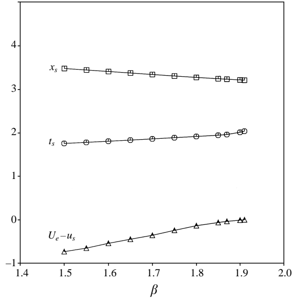
FIGURE 5. Variation of x_s , t_s , U_e(x_s) - u_s with wall speed \beta .
