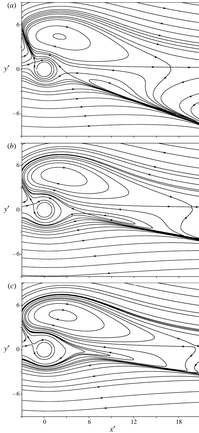
FIGURE 8. Instantaneous streamlines for the cylinder problems at separation for (a) \beta = 1.5 , (b) \beta = 1.7 , (c) \beta = 1.75 ; x' and y' denote Cartesian coordinates.
